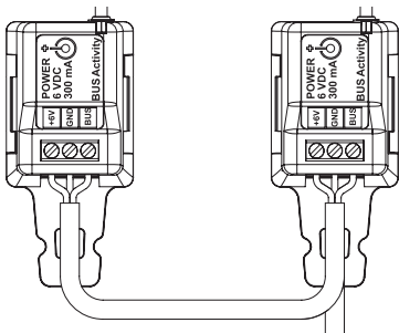
Wired in parallel: +6V to +6V, etc.
